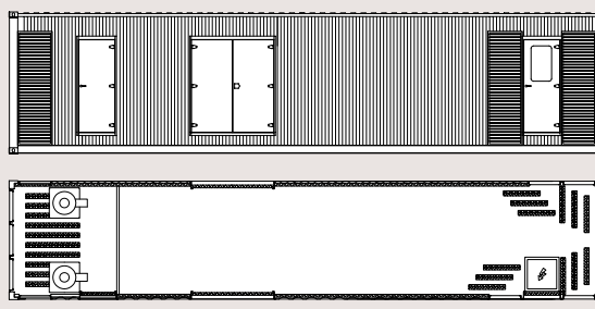
CONTAINER 40'HC
